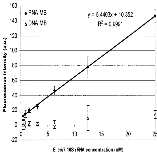
FIG. 2. Quantification of E. coli 16S rRNA with 50 nM PNA and DNA Bact0338 MBs. Concentrations of 16S rRNA in E. coli total RNA extraction were approximately 0 (control), 0.39, 0.78, 1.56, 3.125, 6.25, 12.5, and 25 nM. The MB background fluorescence was subtracted from each sample. a.u. indicates arbitrary units. Each value shown is the mean plus or minus standard deviation of the mean of three replicates.
