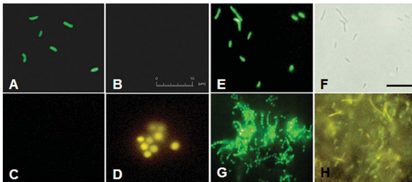
FIG. 3. Epifluorescence micrographs showing the use of DNA MBs and PNA MB to detect bacterial and archaeal cells. Pure culture of E. coli (A and B) and M. acetivorans (C and D) were fixed by using 4% paraformaldehyde and were incubated with DNA MB Bact0338 (A and C) and DNA MB Arch0915 (B and D). The 10- \mu m bar in panel B also applies for panels A, C, and D. Fluorescence micrograph of pure culture of E. coli hybridized with PNA MB Bact0338 (E) and corresponding phase-contrast image (F). Fluorescence micrographs of biomass from UASB reactor incubated with PNA MB Bact0338 (G) and DNA Bact0338 and Arch0915 MBs (H). The bar in panel F corresponds to 10 \mu m and also applies for panels E, G, and H.
