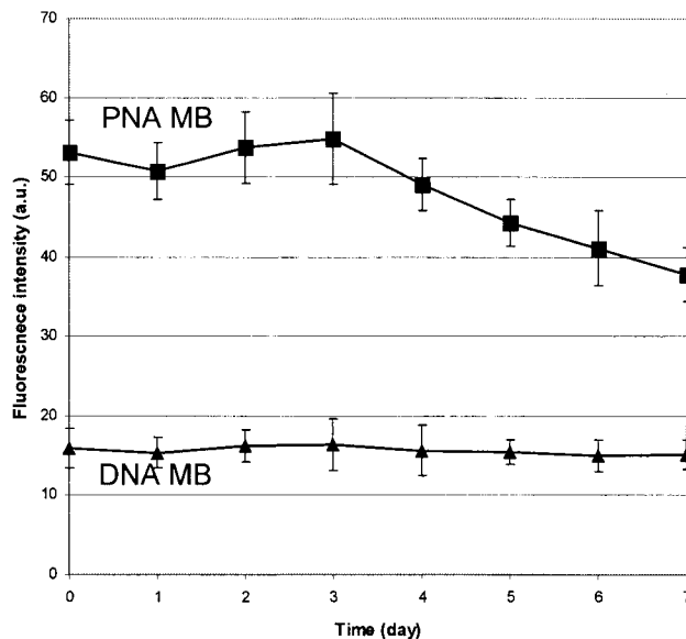
FIG. 6. Study of degradation of cellular E. coli rRNA. Flow cytometry analysis of stationary-phase-harvested cells of E. coli , deprived for different numbers of days of nutrients hybridized with PNA and DNA Bact0338 MBs. a.u. indicates arbitrary units. Each value shown is the mean plus or minus standard deviation of the mean of three replicates.
