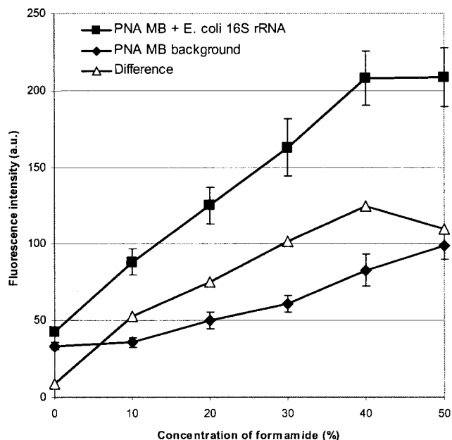
FIG. 1. Optimization of formamide concentration in Tris-HCl-NaCl hybridization buffer for PNA MB Bact0338 to detect rRNA in solution. The hybridization buffer contained 25 mM Tris-HCl and 100 mM NaCl and different concentrations of formamide. Each value shown is the mean plus or minus standard deviation of the mean of three replicates. PNA MB background represents fluorescence intensity of 50 nM PNA MB Bact0338 (control); PNA MB + E. coli 16S rRNA indicates fluorescence intensity of 50 nM PNA MB Bact0338 incubated with total RNA extracted from a pure culture of E. coli containing around 25 nM 16S rRNA; Difference refers to the absolute value of fluorescence intensity of hybridization signals obtained by subtracting results obtained with the PNA MB alone from hybridization signals. a.u. indicates arbitrary units.
