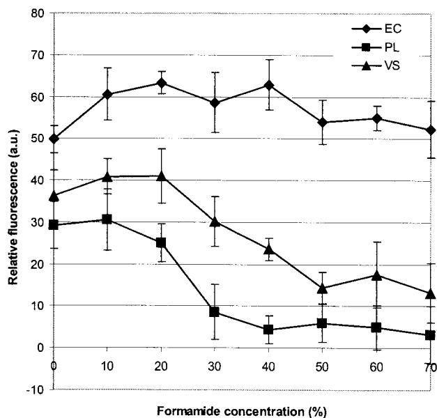
FIG. 5. Formamide and specificity study for PNA MB Bact0338. Flow cytometry analysis of E. coli (EC, perfect match), V. spinosum (VS, two mismatches), and P. limnophilus (PL, three mismatches) cells hybridized with 50 nM PNA MB Bact0338 in hybridization buffer containing different concentrations of formamide (0 to 70% [vol/vol]). a.u. indicates arbitrary units. Each value shown is the mean plus or minus standard deviation of the mean of three replicates.
