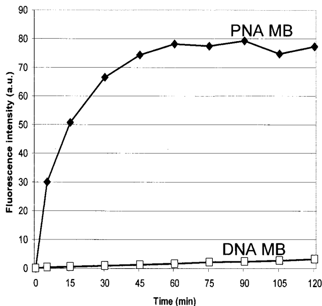
FIG. 4. Flow cytometry analysis of hybridization kinetics for mid-log-phase-harvested cells of E. coli hybridized for different time periods with PNA and DNA Bact0338 MBs. a.u. indicates arbitrary units.
