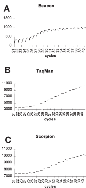
Figure 4. Fluorescence accumulation patterns for three fluorescence signaling methods. The accumulation of fluorescence throughout each 60°C anneal extend segment was monitored for three signal generation technologies: (A) Molecular Beacons, (B) TaqMan, and (C) Scorpions.
