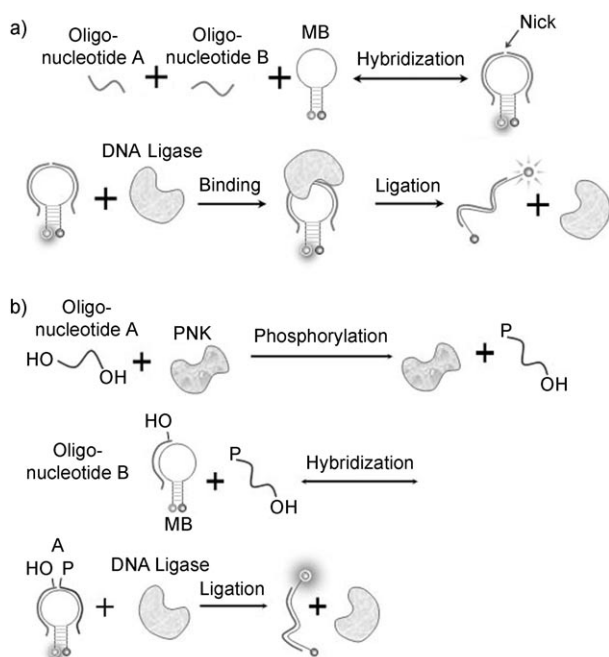
Figure 5. Application of MBs in phosphorylation and ligation studies. a) Real-time monitoring of nucleic acid ligation: Two oligonucleotides that are complementary to opposite halves of the MB loop hybridize with the MB, whereby a nick is formed, and the stem may be opened slightly. The DNA ligase binds to the nick and catalyzes the ligation of the two short oligonucleotides to form a longer oligonucleotide. The ligation product hybridizes with the MB to restore fluorescence. b) Monitoring of nucleic acid phosphorylation: Oligonucleotide A is first phosphorylated at the 5'-hydroxy group by the polynucleotide kinase. The nick formed upon the hybridization of oligonucleotide B and phosphorylated oligonucleotide A with MB can be sealed by the DNA ligase, whereupon the stem helix of the MB is opened, and fluorescence is restored.
