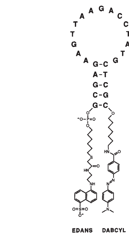
Figure 2. Structure of molecular beacon A. This oligodeoxyribonucleotide (represented by bold letters) consists of a 15-nucleotide-long probe sequence embedded within two complementary 5-nucleotide-long arm sequences. The fluorophore, EDANS, is joined to the 5'-terminal phosphate by a -(CH_2)_6-S-CH_2-CO- linker; and the quencher, DABCYL, is joined to the 39-terminal hydroxyl group by a -(CH_2)_7-NH- linker. Although the terminal adducts are schematically depicted on a larger scale than the nucleotide sequence, each adduct is approximately the same size as a single nucleotide.
