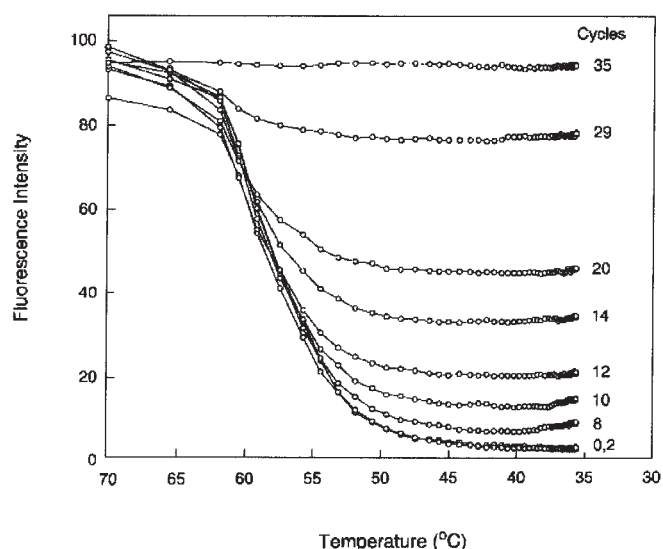
Figure 6. Demonstration that molecular beacons can be used to measure the amount of DNA synthesized in a homogeneous reaction. A polymerase chain reaction was carried out in the presence of molecular beacon B, which was complementary to a sequence in the middle of the DNA being amplified. The reaction was divided into several aliquots. After a predetermined number of amplification cycles, each aliquot was heated to 100°C, placed in a cuvette thermostated at 37°C, and its fluorescence was recorded as the temperature dropped rapidly (65°C to 40°C in 2 min). At high temperatures, the molecular beacons were denatured and they fluoresced brightly. As the temperature dropped, they renatured and became dark, unless there were amplified DNA strands present, in which case they formed fluorescent hybrids. As more cycles of amplification were carried out, the fraction of molecular beacons that remained fluorescent increased, reflecting the increase in the amount of DNA synthesized. A comparison of the fluorescence intensity in each aliquot at 37°C and the amount of DNA synthesized (as determined by polyacrylamide gel electrophoresis and ethidium bromide staining) indicated that there is a strong correlation between these two detection methods and they are about equally sensitive. Furthermore, there was no detectable degradation of the molecular beacons after 35 cycles of amplification.
