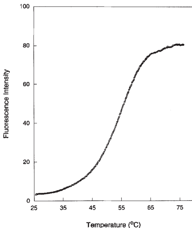
Figure 3. Thermal transition profile of a molecular beacon. The fluorescence intensity of a solution containing molecular beacon A is plotted as a function of temperature on a linear scale from 0 to 100. The minimum intensity was determined from the fluorescence of the buffer alone, and the maximum intensity was determined by adding an excess of target strands to the solution. The increase in fluorescence seen when the temperature was raised is due to a change in the conformation of the molecular beacons from a stem-and-loop structure to a random coil. Because the maximum fluorescence that occurs upon thermal denaturation is lower than the amount of fluorescence that occurs when the probes are fully extended by hybridization to a target, it can be inferred that molecular beacon A is so small that the fluorophore at one end of the random coil occasionally interacts with the quencher at the other end before its stored energy is released as fluorescent light.
