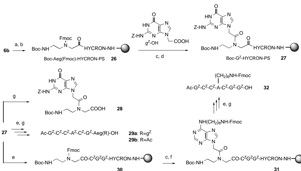
Scheme 7. a) aminomethyl polystyrene, HBTU, i Pr 2 NEt, HOBT, DMF; b) Ac 2 O, Pyr; c) DMF/morpholine; d) HATU, i Pr 2 NEt, DMF; e) Boc/Z-PNA solid-phase synthesis (see Scheme 5); f) 11 , HATU, i Pr 2 NEt, DMF; g) [Pd(PPh 3 ) 4 ], morpholine (MeNHP for 32 ), DMSO, DMF ( 28 , 61%; 29a , 36%; 29b , 39%; 32 , 50%). (Aeg = aminoethylglycine, HATU = O -(1-oxy-7-azabenzotriazole-1-yl)- N,N,N',N' -tetramethyl-uronium hexafluorophosphate, PS = polystyrene).
