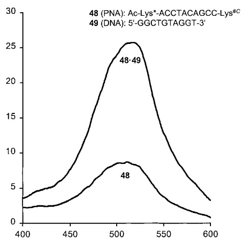
Figure 7. Fluorescence spectra (arbitrary units) of the terminally labelled PNA-probe 48 as single strand and in complex with DNA 49 (Lys* = Cys(Dans), Lys # = Lys(DABCYL)). Measurement conditions: 100 mM NaCl, 10 mM NaH 2 PO 4 , pH 7, 298 K, 1 μM in 48 , 1 μM in 49 when added, excitation at 330 nm.
