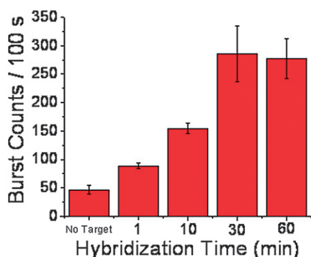
Fig. 5 Number of fluorescent bursts detected versus hybridization time (5 pM targets, 10 pM probe) within the device. Hybridization time follows a 15 s mixing period using the rotary pump and a 5 s incubation at 80 °C.
