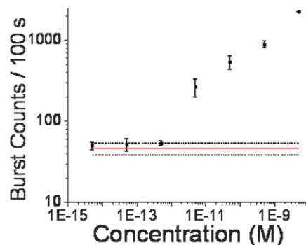
Fig. 4 Calibration curve of fluorescence burst counts versus target concentration loaded into the SMD rotary chamber 23 without evaporation-based accumulation (10 pM molecular beacon concentration). The solid line represents the average number of fluorescent bursts from the no target control (dotted line equals one standard deviation from an average of four measurements).
