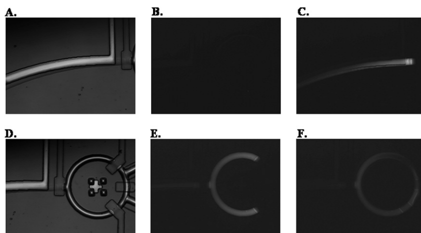
Fig. 2 (A and B) Photo- and fluorescence micrographs of the accumulation zone just prior to the closed accumulation valve at time 0 after loading the evaporator coil with 500 nM fluorescently-labeled DNA sequences. (C) Fluorescence micrograph showing target accumulation after 6 hours of evaporation in the 1000 mm membrane pervaporator with 20 PSI nitrogen pressure and at room temperature. (D) Photomicrograph of the SMD rotary chamber just prior to sample injection with valves bisecting the chamber into analyte (left three-quarters) and probe/buffer (right one-quarter) compartments. (E) Accumulated model target from Fig. 2C is injected into the rotary chamber along with DI water in the probe/buffer section. (F) Mixing of the contents shown in Fig. 2E for 1 s using the rotary pump at 10 Hz, mixing at the 100 Hz pump rate was complete within 5 s (data not shown).
