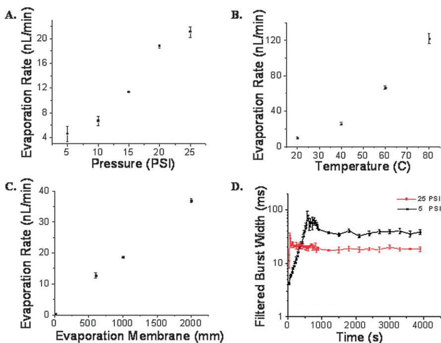
Fig. 3 (A, B, and C) Bulk evaporation rates versus evaporation pressure (A), microdevice temperature (B), and evaporation membrane length (C). Pressure data were taken using a 1000 mm membrane at room temperature. Temperature data were taken using a 1000 mm membrane at 25 PSI, while evaporation length data were taken at room temperature and 25 PSI. (D) Time trace of the measured fluorescent burst duration of tetraspec beads at the start of the evaporation channel at two different evaporation pressures (25 and 5 PSI). Large fluctuations at low pressure are due to evaporation membrane vibration upon initiation of nitrogen flow. Points for A, B, and C are mean evaporation rates from a single device after three separate 2 h measurements \pm standard error.
