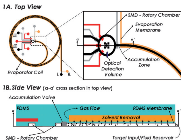
Fig. 1 (A) Schematic of the combined micro-evaporator/rotary SMD microdevice. The control layer (lighter grey) shows the evaporation membrane, rotary pump, and isolation valves. Target accumulation is accomplished by solvent removal from the fluidic layer (black, inlet labeled i.) through the pervaporation membrane (inlet labeled ii.). Following target accumulation the concentrated sample plug is transferred to the SMD rotary chamber for probe hybridization and detection; probes and hybridization buffer are introduced through separate inlets (labeled iii.). (B) Side view of the operating micro-evaporator, prior to sample transfer into the detection chamber. Solvent removal through the pervaporation membrane must be compensated by convection from the sample reservoir, while actuation of the accumulation valve enables target collection at the dead end.
