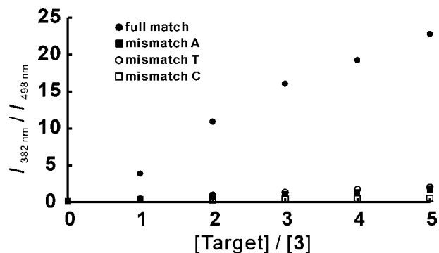
FIGURE 5. Discrimination of complementary target DNAs from their single-nucleotide mismatches. A ratio of I_{382\text{nm}}/I_{498\text{nm}} for 3 ( 3 ), 5 nM; [\text{MgCl}_2] , 5 mM; [\text{KCl}] , 50 mM; [\text{Tris-HCl}] , 20 mM, at pH 8.0 including 20% DMF) was plotted as a function of [\text{target}]/[\mathbf{3}] . Closed circle, closed square, open circle, and open square correspond to the full-match 5 and the single-nucleotide mismatches 7 , 8 , and 9 , respectively.
