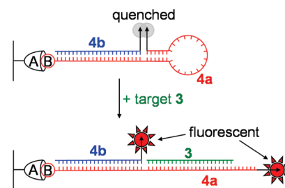
Figure 4. Schematic illustrating closed and open conformations of the biotin(B)-NeutrAvidin(A) surface-immobilized two-piece SQUID MB 4 used for SM imaging.
