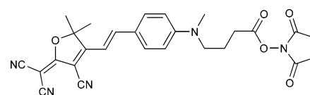
Figure 1. Structure of NHS ester-functionalized DCDHF fluorophore 1 .
